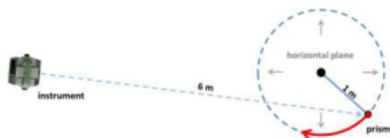
Figure 14 - Test setup to check the distance synchronisation (top view).
