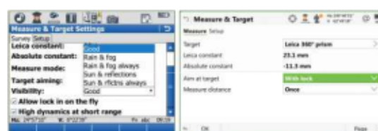
Figure 6 - Overview of the manual settings in SmartWorx Viva with ATR (left) and Leica Captivate with ATRplus (right).
